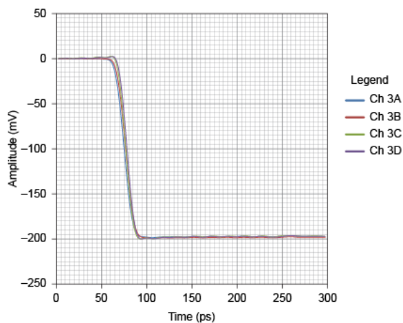
Figure 2. Options 32F, 32M, 34F, and 34M with TDR Calibration (Characteristic)
